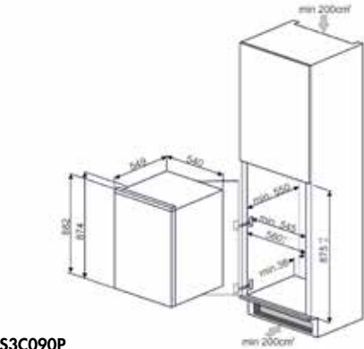
S3C090P
