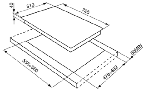
P272XGH
