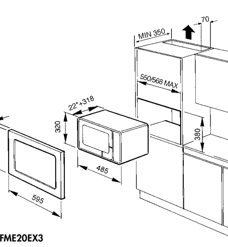
FME20EX3
