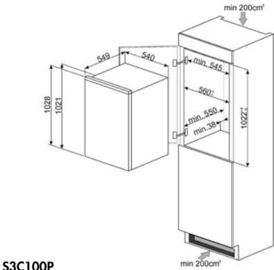
S3C100P
