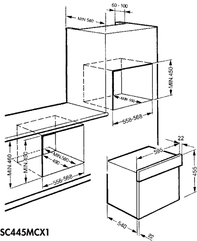
SC445MCX1
