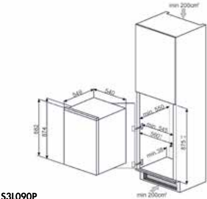
S3L090P
