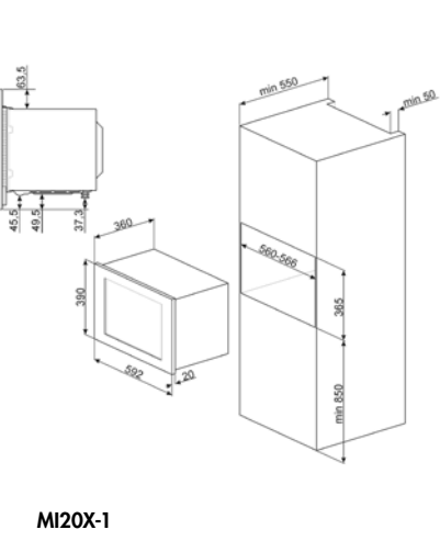
MI20X-1
