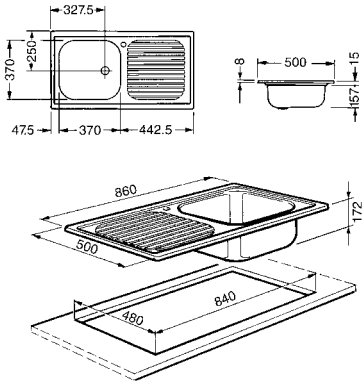
LX861S-2 LX861D-2
