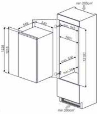
S3L120P
