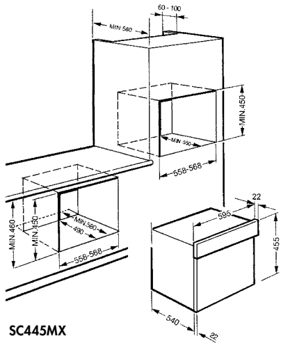
SC445MX
