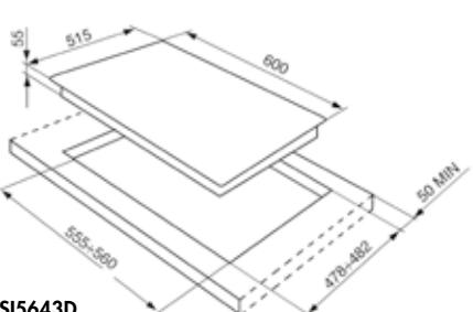
SI5643D
