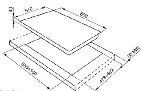
P261XGH
