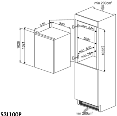
S3L100P
