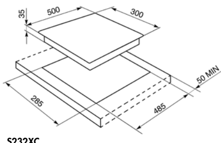
S232XC
